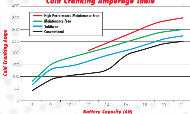
Cold Cranking Amperage Table
