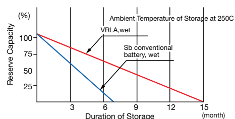
Self Discharge
