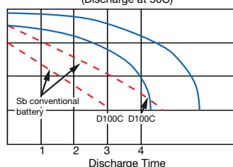
High Rate Discharge Performance (Discharge at 50C)
